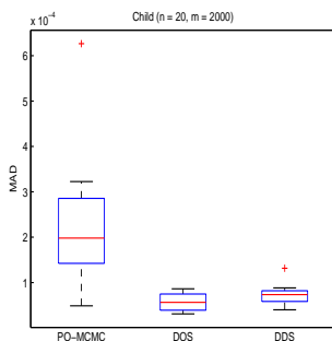
Figure 48: Boxplot of the MAD Performance of the PO-MCMC, the DOS, and the DDS for Child ( m = 2000 )
