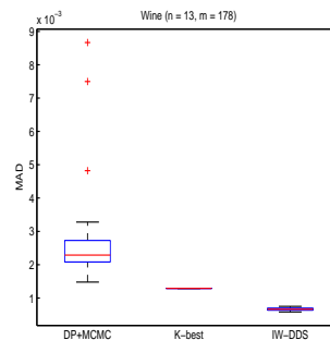
Figure 52: Boxplot of the MAD Performance of the DP+MCMC, the K -best, and the IW-DDS for Wine
