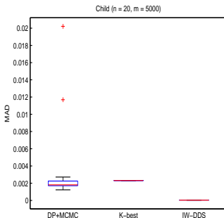
Figure 82: Boxplot of the MAD Performance of the DP+MCMC, the K -best, and the IW-DDS for Child ( m = 5000 )
