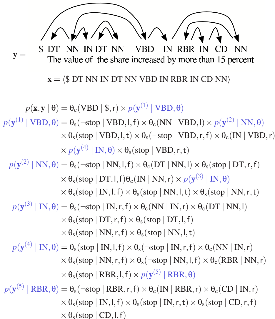
Figure 1: An example of a dependency tree (derivation \mathbf{y} ). and its probability. The part-of-speech tags NN, VBD, DT, CD, RBR, and IN denote noun, past-tense verb, determiner, number, comparative adverb, and preposition, respectively, following Penn Treebank conventions. We break the probability of the tree down into recursive parts, one per head word, marked in blue (lighter). l, r, t, and f denote left, right, true, and false, respectively (see Equation 4).
