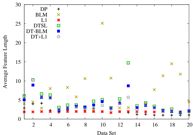
Figure 6: Average feature length for each algorithm on each data set.
