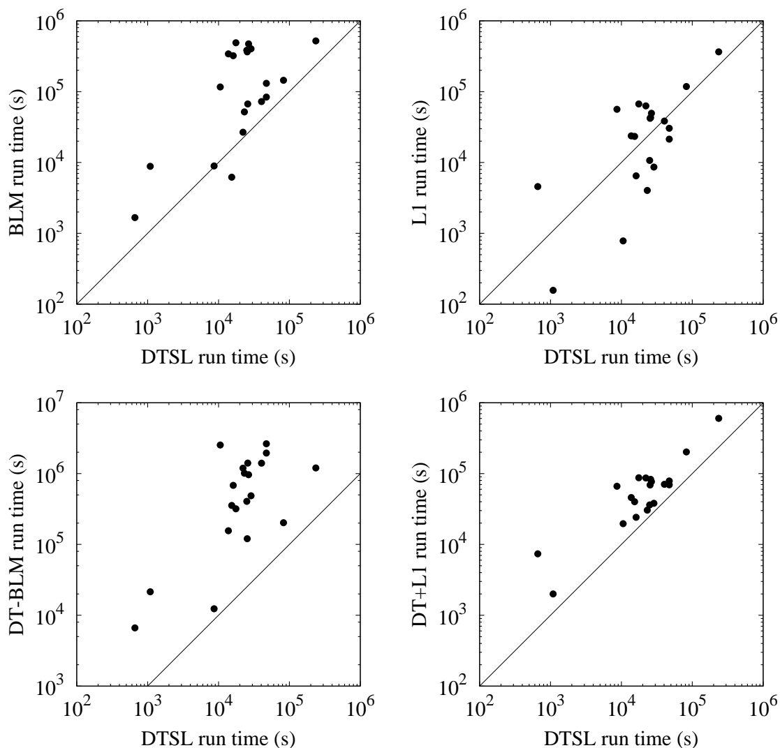
Figure 10: Running time on each data set in seconds (y-axis) relative to DTSL’s running time (x-axis). Points below the line y=x represent data sets where DTSL was slower than the other algorithm. All times include tuning.
