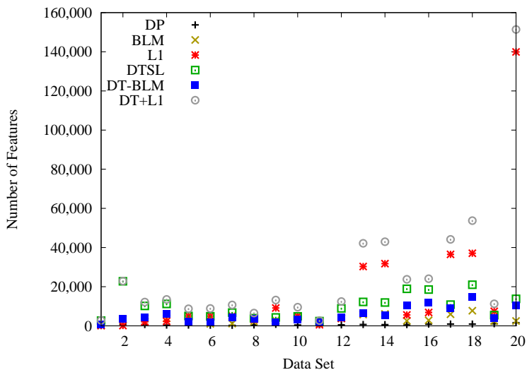
Figure 7: Number of features for each algorithm on each data set.
