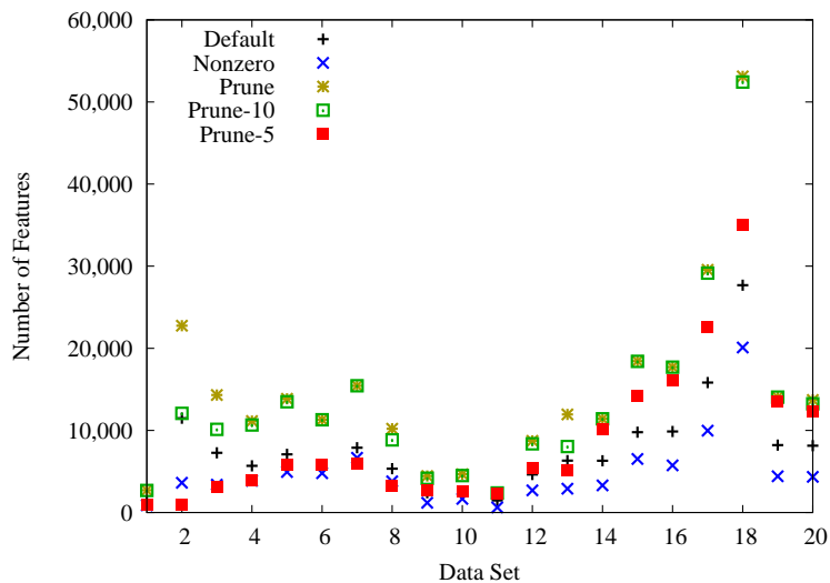
Figure 4: Number of features for each DTSL feature generation method on each data set.
