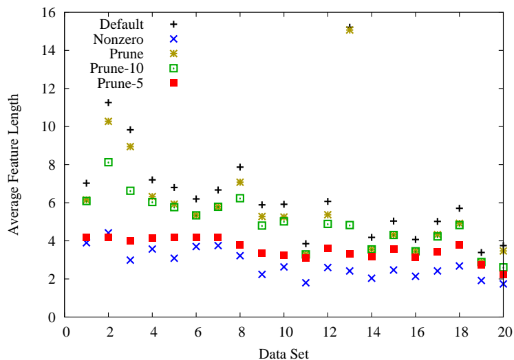
Figure 3: Average feature length for each DTSL feature generation method on each data set.
