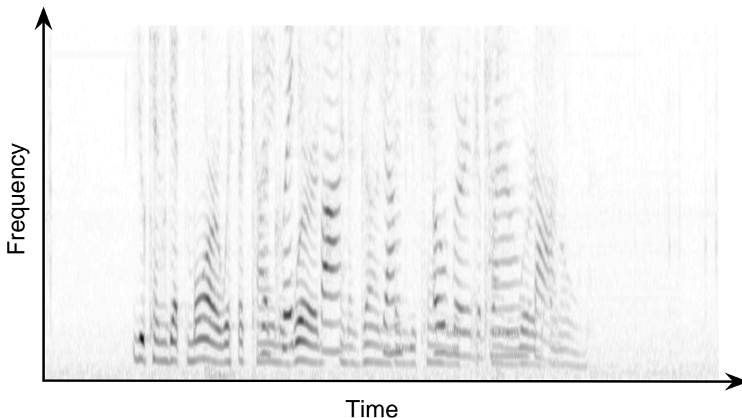
Figure 9: Spectrogram of speech (two simultaneous English speakers). The gray intensity is proportional to the amplitude of the spectrogram.
